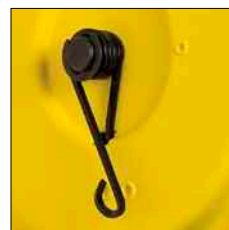
Adjustment of spring tension Model YFS-03/04/05 with central shaft and spring lever
